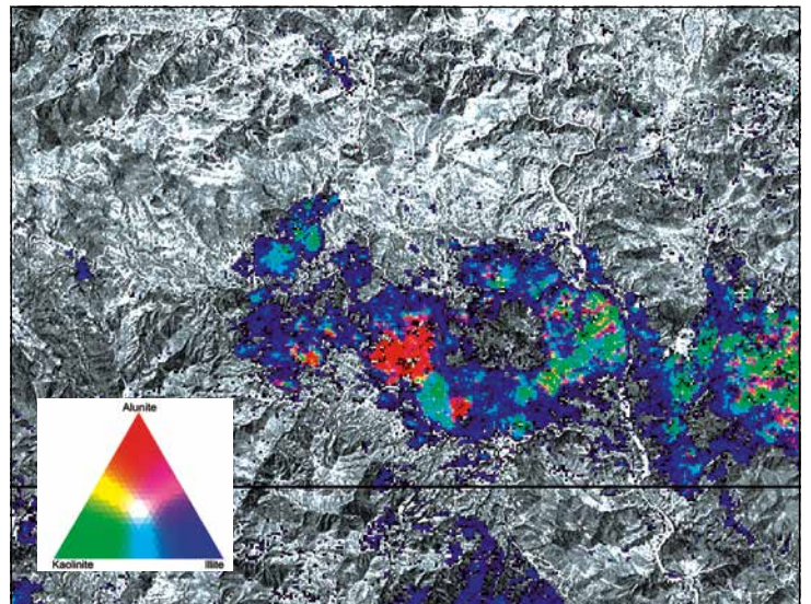
The image above shows a mineral mapping product derived from the ASTER satellite sensor. Different colours indicate concentrations of alunite, kaolinite, and illite.
