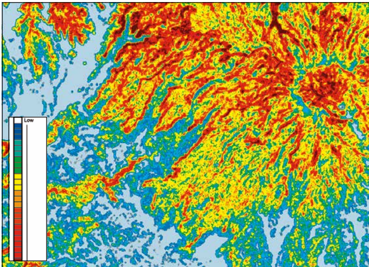
In the terrain complexity image above, less-complex areas are shown in gray and blue. Higher terrain complexity is shown in orange and red.
