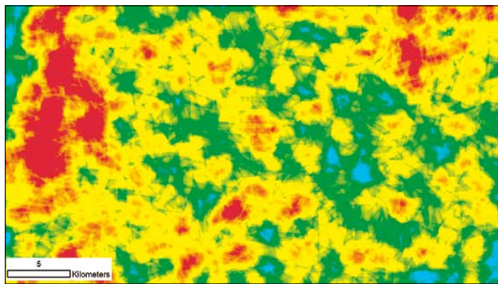
In the Density Map above, the gradation in colour from red to blue represents the highest to lowest density of fractures derived from a variety of image sources.
