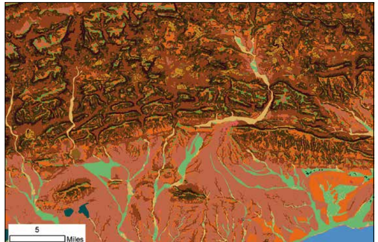
The image above shows an example of a 90-metre model of soil texture. Blue indicates water, and each of the other colours represent classes from the American Society of Testing and Materials (ASTM) Unified Soil Classification System (USCS).
