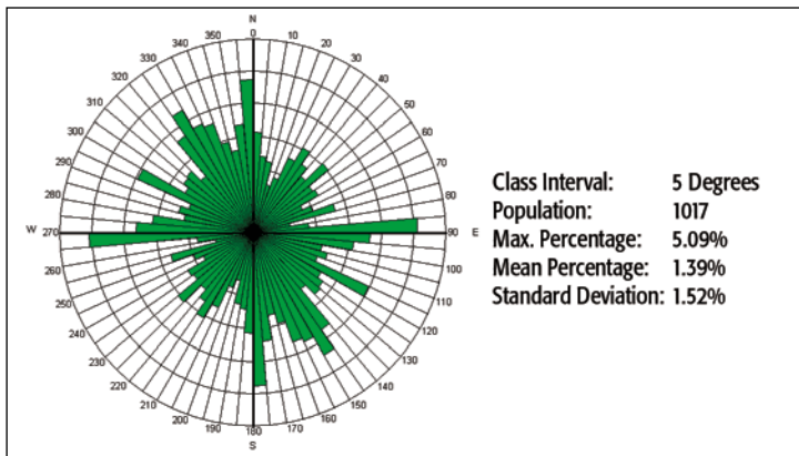
The image above shows a Rose Diagram, where green indicates the relative number of fractures at each orientation shown on the circular graph.
